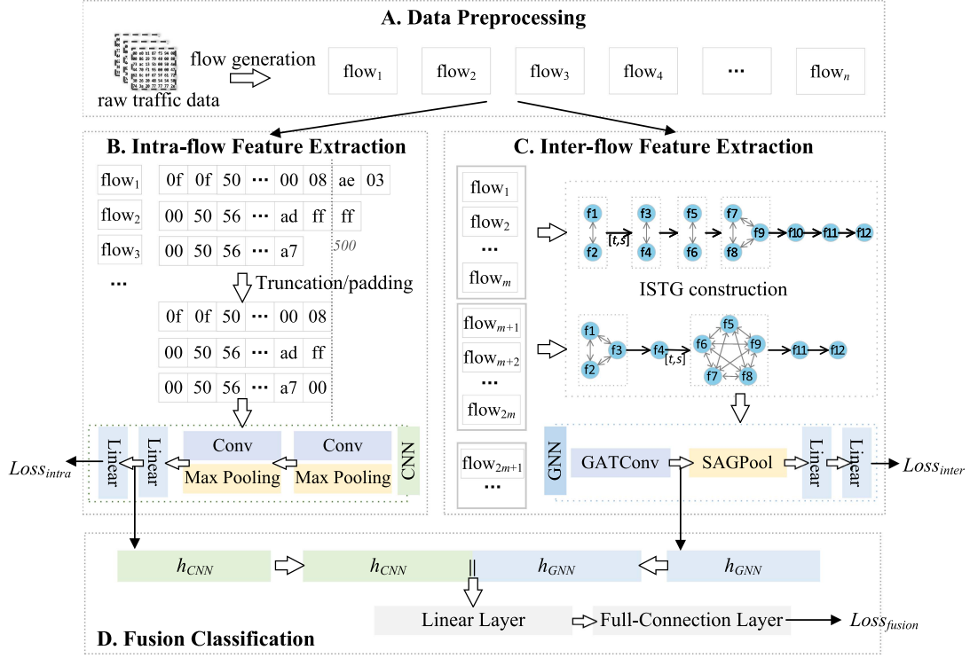
Fig. 2. The system framework of the proposed IF 2 -STG, consisting of four modules: (a) Data Preprocessing provides features required for subsequent modules, (b) Intra-flow Feature Extraction and (c) Inter-flow Feature Extraction learn the representations of two modalities, and (d) Fusion Classification combines these representations for final intrusion detection.
