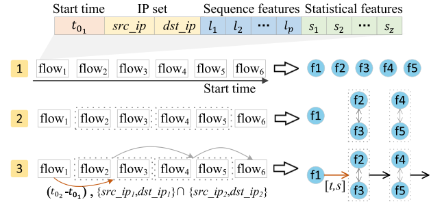
Fig. 3. An example of ISTG construction (assuming m=6 ), comprising three key steps: 1) Flow Sorting: Sorting the m flows by their start times, corresponding to the node order in ISTG. Each flow requires features such as start time, IP set, sequence features, and statistical features. 2) Concurrent Flow Grouping: Flows within each dashed box form a concurrent group, and bidirectional edges connect concurrent flows in ISTG. 3) Spatio-temporal Relationship Calculating: Nodes or groups in ISTG are sequentially linked with unidirectional edges weighted by 2D spatio-temporal vectors [t, s] .
