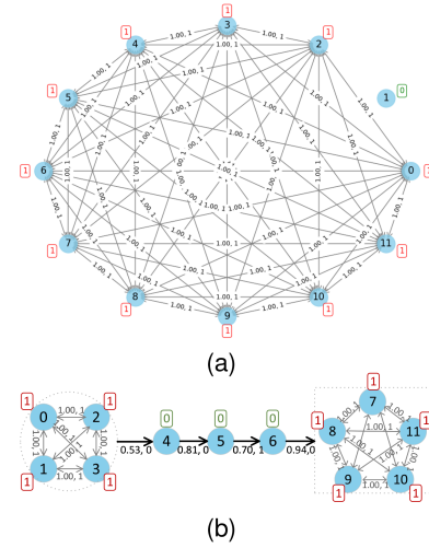
Fig. 13. ISTG corresponding to mixed traffic.
