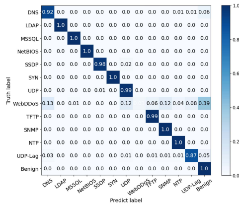
(a) CIC-DDoS2019
