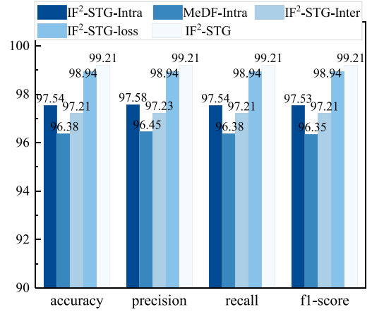
Fig. 7. Ablation study results.
