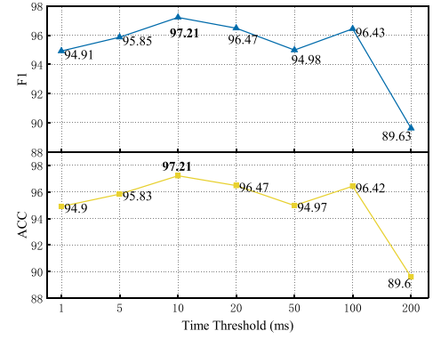
Fig. 8. The Impact of Time Threshold on Classification Performance.
