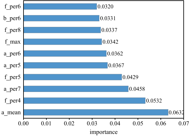
Fig. 4. Top 10 most important statistical features ranked using random forest.
