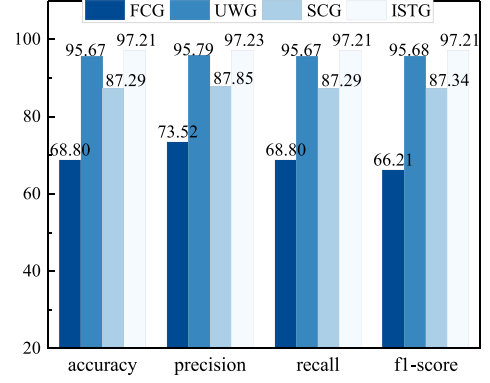
Fig. 9. The Impact of ISTG Construction Scheme on Classification Performance.
