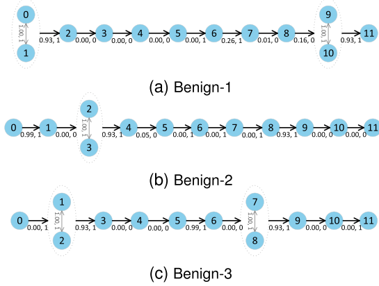
Fig. 10. ISTG corresponding to benign traffic.
