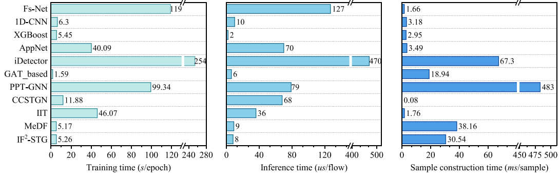
Fig. 6. Comparison of time cost of each baseline model.
