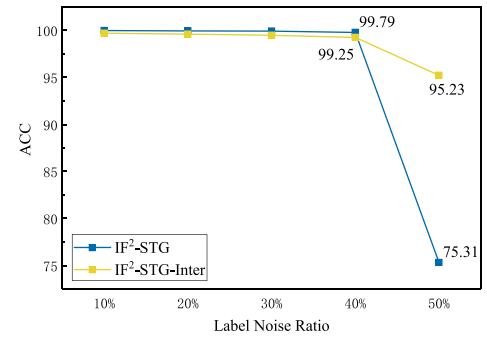
Fig. 14. The Impact of labeling noise on Classification Accuracy.
