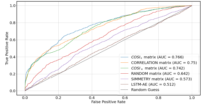
Fig. 5. AUC ROC curve results for Cisco dataset.
