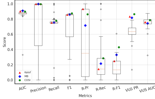
Fig. 7. Graph structure comparison using GDN.
