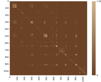
Fig. 4. Adjacency matrix of COSI_{\times} graph - Th: 0.9.
