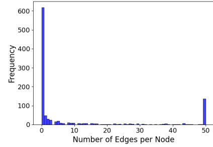
Fig. 3. Edges number distribution of COSI_{\times} Top 50. (5G3E).
