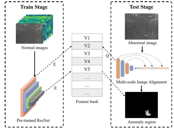
Fig. 7. Pipeline of SPADE. In the training stage, SPADE employs a pretrained ResNet to extract features from normal images. The features are subsequently stored in a feature bank. During the test stage, a multiscale image alignment is utilized for anomaly localization. This involves querying the features in the feature bank to generate an anomaly map. In the illustration, “E” denotes “extract features” and “Q” signifies “query.”
