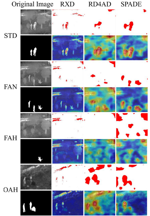
Fig. 10. Performances of the traditional and deep learning detection algorithms on the fused dataset. In comparison with the single modality, high anomaly scores (i.e., the hotter regions) in the heat maps are more concentrated on the person to be rescued, with diminished distribution over the background. Furthermore, in the binary maps, the anomaly regions cover the ground truth more comprehensively, demonstrating the improvements with fusion.
