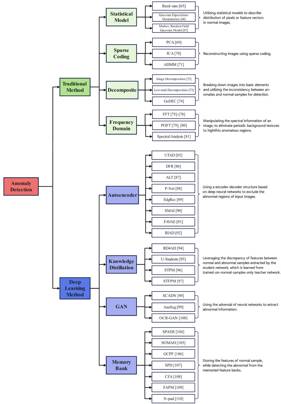
Fig. 3. Anomaly detection methods overview.
