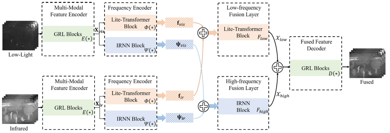
Fig. 2. Architecture of the proposed dual-stream multimodal fusion model based on frequency-domain feature decomposition.
