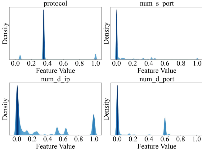
Fig. 4. The density distribution of Mawi datasets extracted by FlowVision. The x-axis represents the feature value, while the y-axis indicates the density, and darker colors correspond to higher density.
