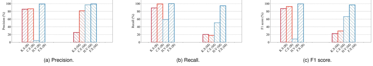
Fig. 6. Comparative experiments with SOTA methods on the MAWI dataset (2021/3/1).
