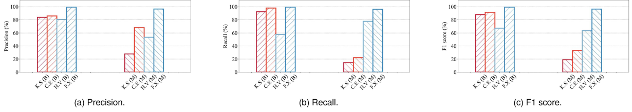
Fig. 7. Comparative experiments with SOTA methods on the MAWI dataset (2023/6/3).
