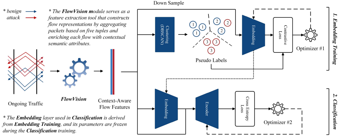
Fig. 2. The framework of FlowXpert.
