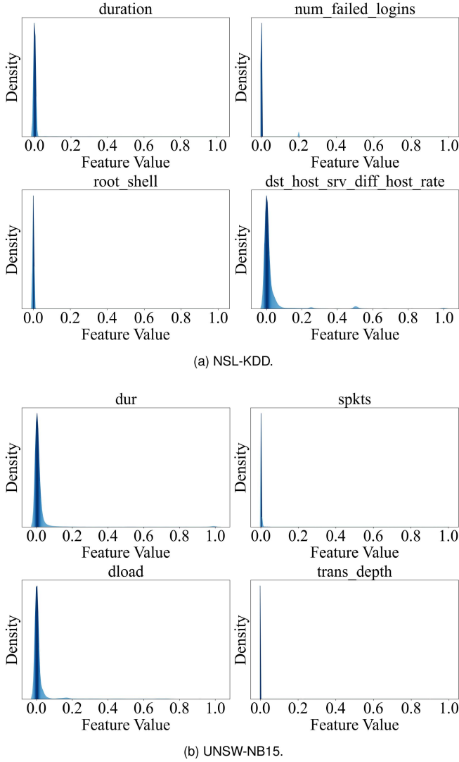
Fig. 1. The density distribution of NSL-KDD and UNSW-NB15 datasets. The x-axis represents the feature value, while the y-axis indicates the density, and darker colors correspond to higher density.
