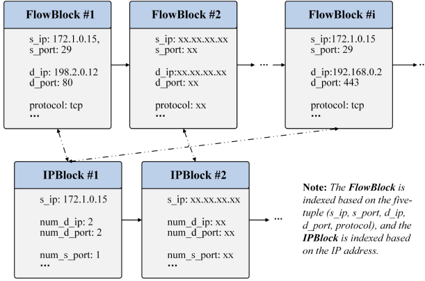
Fig. 3. The data structure of FlowVision .
