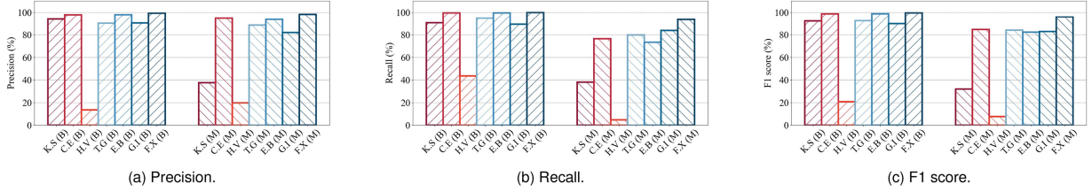
Fig. 8. Comparative experiments with SOTA methods on the CICIDS-2017 dataset.
