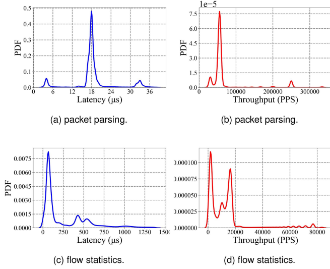
Fig. 9. Performance test of FlowVision on the MAWI dataset.
