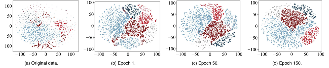
Fig. 5. Visualization of embedded representations using t-SNE on the MAWI dataset, illustrating the evolution of the proposed method during training (the different colors in the figure represent different pseudo labels).
