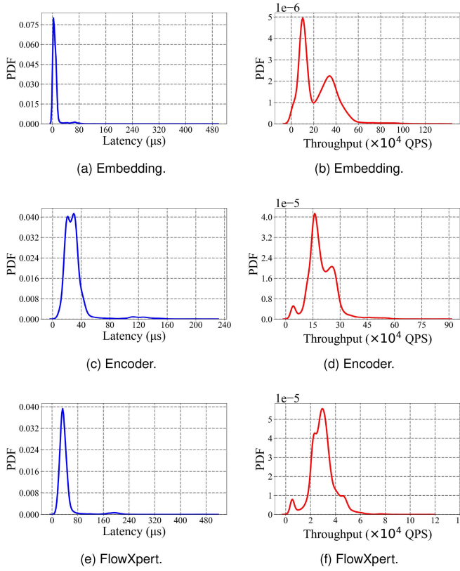
Fig. 10. Performance test of FlowXpert on the MAWI dataset.
