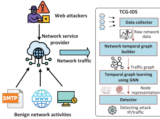
Fig. 1. Threat model.
