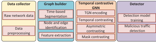
Fig. 2. Overview of TCG-IDS.
