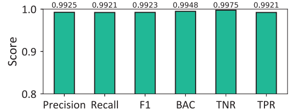
Fig. 10. Overall performance under NF-CSE-CIC-IDS2018-v2.
