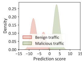
Fig. 8. Distribution of prediction score under NF-CSE-CIC-IDS2018-v2.
