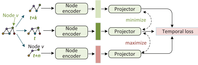
Fig. 3. Illustration of temporal contrasting.
