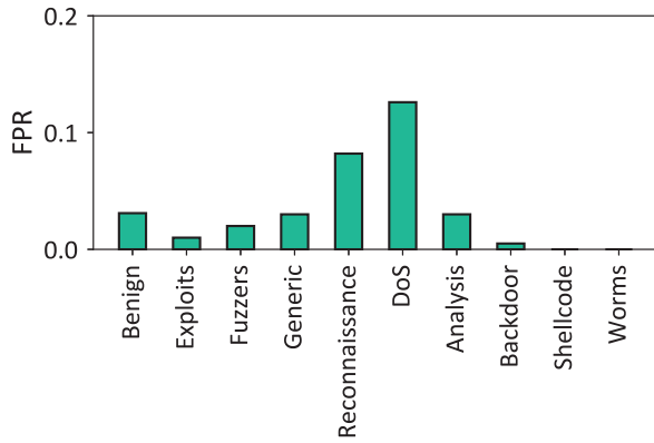
Fig. 13. Multi-class FPR under NF-UNSW-NB15-v2.
