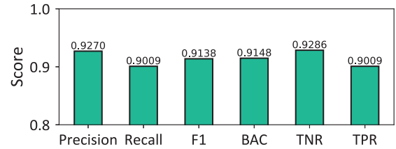
Fig. 11. Overall performance under NF-UNSW-NB15-v2.
