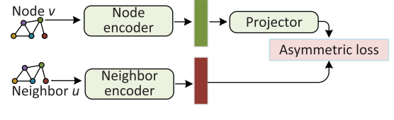
Fig. 4. Illustration of asymmetric contrasting.
