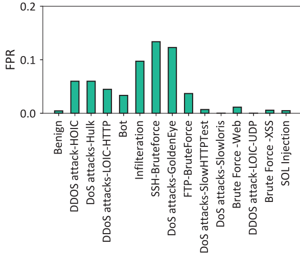
Fig. 12. Multi-class FPR under NF-CSE-CIC-IDS2018-v2.
