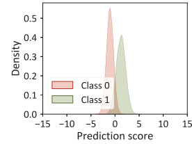
Fig. 9. Distribution of prediction score under NF-UNSW-NB15-v2.
