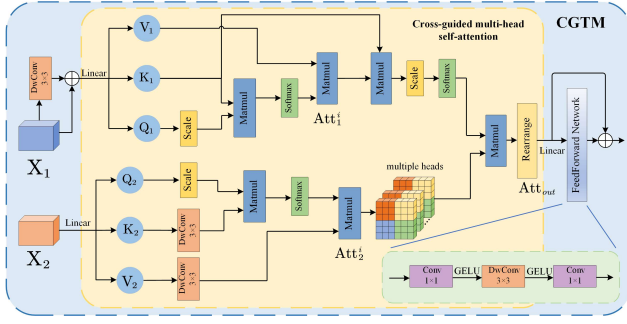
Fig. 4. Schematic of CGTM.
