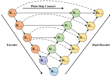
Fig. 2. Illustration of our dual-decoder structure.
