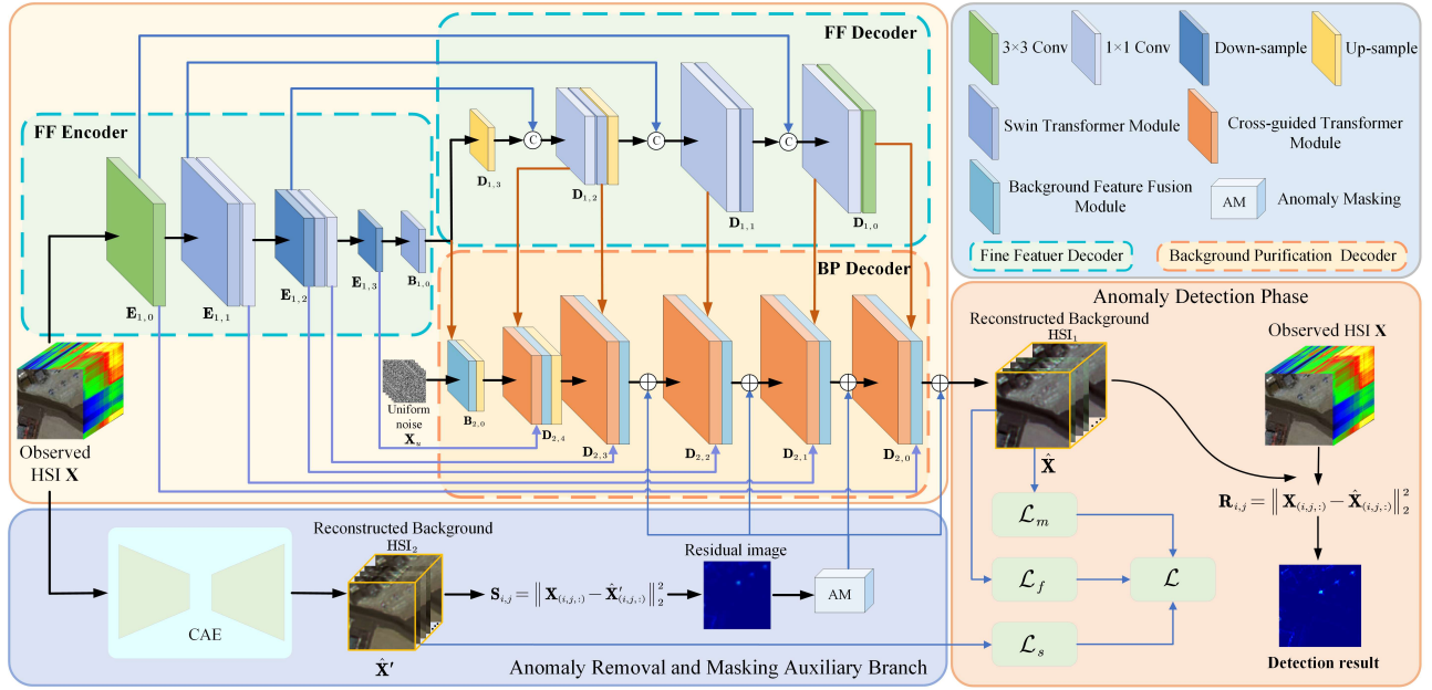
Fig. 1. D 3 Former for HAD. The observed HSI first undergoes the FF encoding and decoding process, and the uniform noise is fed into the lower layer BPD to simulate anomaly-free input. CGTM enhances feature representation in background regions, while ARMAB reduces the weight of anomalous pixels. During the detection stage, BFFM performs cross-stage feature fusion of background information from different layers to obtain the reconstructed “anomaly-free” background HSI 1 , and the final detection result is acquired via the difference between the “anomaly-free” background HSI 1 and the original HSI.
