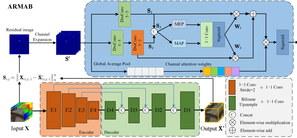
Fig. 3. Illustration of ARMAB.
