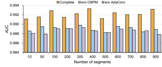
Fig. 9. Detection performance of SuperAD with different numbers of superpixel segments on San Diego dataset.
