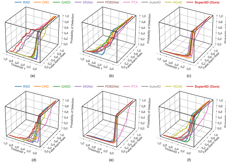
Fig. 5. 3D-ROC curves of the 9 considered detectors on (a) San Diego, (b) Texas Coast, (c) ABU-Urban-1, (d) ABU-Urban-2, (e) ABU-Urban-3, and (f) ABU-Urban-4.
