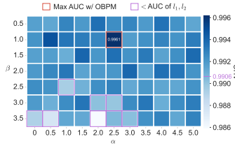
Fig. 8. Ablation studies and parameter analysis conducted on San Diego dataset for OBPM.
