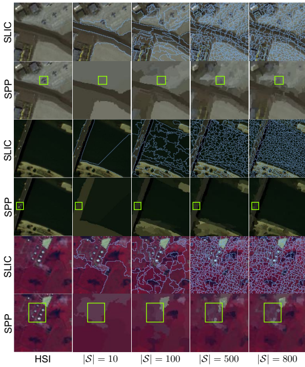
Fig. 10. Visualization of superpixel pooling with different numbers of superpixels. Bright boxes highlight the anomalous regions.
