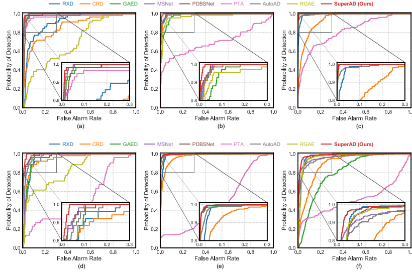
Fig. 3. ROC curves of the 9 considered detectors on (a) San Diego, (b) Texas Coast, (c) ABU-Urban-1, (d) ABU-Urban-2, (e) ABU-Urban-3, and (f) ABU-Urban-4.
