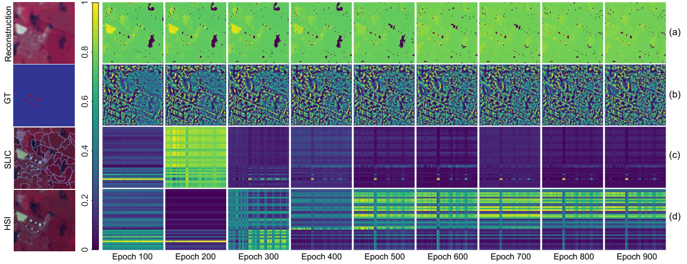
Fig. 12. Visualization of training process: (a) OBPM gradients visualization. (b) AdaConv pixel utilization visualization. (c) and (d) SPP self-attention score matrices visualization of the last and the first layer.
