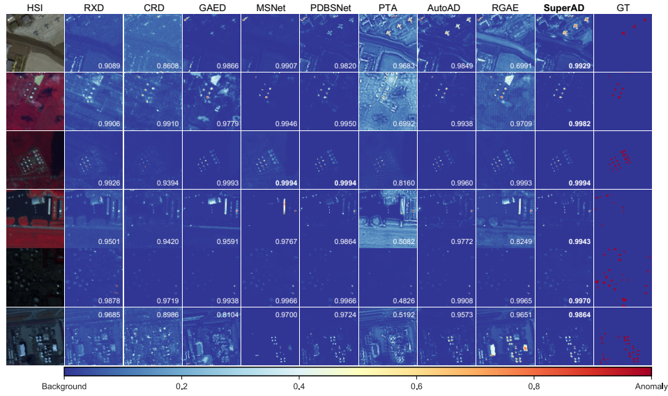
Fig. 6. Visualization of detection results of the 9 considered detectors on (from top to bottom) San Diego, Texas Coast, ABU-Urban-1, ABU-Urban-2, ABU-Urban-3, and ABU-Urban-4.
