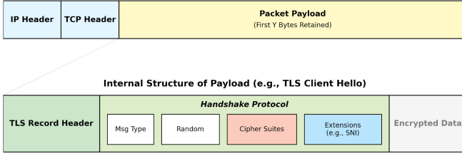
Fig. 4. Illustration of observable unencrypted metadata (e.g., Extensions) within the payload bytes of encrypted traffic.
