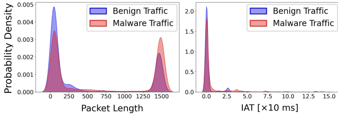
Fig. 1. The KDE of malware and benign traffic across packet length and IAT in CTU-Malware dataset [19].
