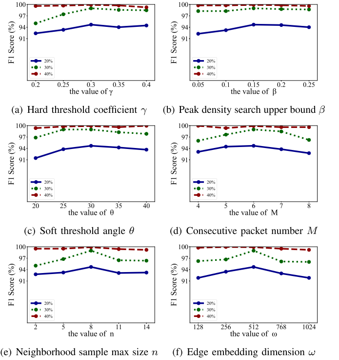
Fig. 8. The detection F1 (%) of different parameter settings at different loading ratios of malware in D_3 .
