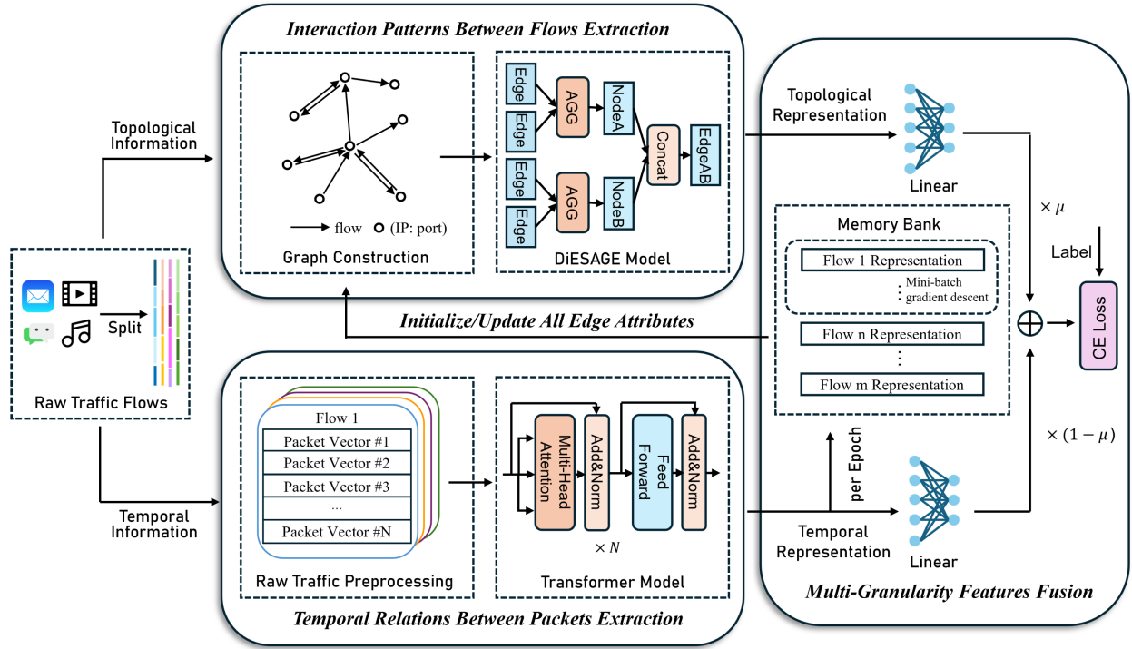
Fig. 1. The overview of proposed BPF-DAG Framework. The lower part illustrates how raw byte packet sequences are input into a Transformer to learn temporal representations. The upper part shows that network connectivity information, combined with the learnable temporal representations, is used to construct graphs, which are then processed by DiESAGE to capture topological representations. The left part details the multi-granularity feature fusion process. During the joint training of DiESAGE and the Transformer, the graph is dynamically updated by iteratively assigning edge attributes based on the evolving temporal representations. The Memory Bank technique is used to decouple the training batch size from the total number of edges. The specific module configurations and parameters are presented in Figure 4 and Table III.
