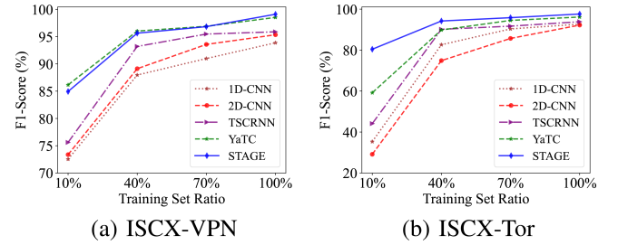
Fig. 9. Comparison results in few-shot settings on ISCX-VPN and ISCX-Tor datasets.
