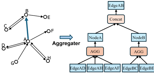
Fig. 3. The illustration of the DiESAGE model in 1-hop propagation scenario.
