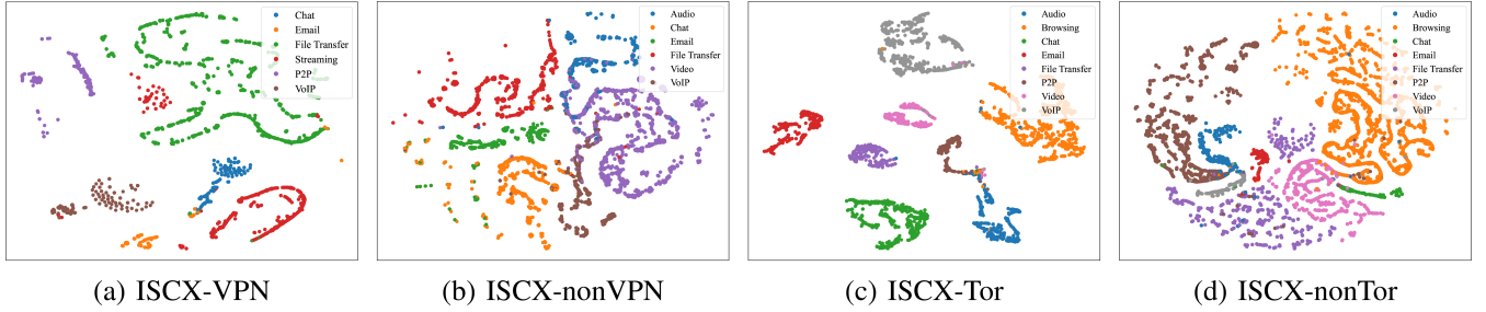
Fig. 8. t-SNE Visualization of the proposed BPF-DAG method on four datasets.
