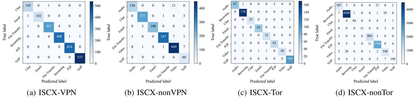
Fig. 5. Confusion matrices of BPF-DAG on four datasets.
