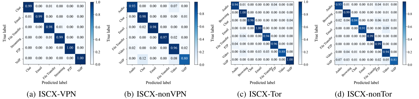
Fig. 6. Normalized confusion matrices of BPF-DAG on four datasets.
