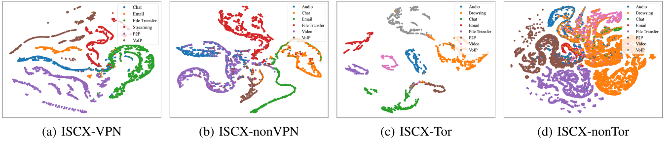
Fig. 7. t-SNE Visualization of ablation study without using topological features on four datasets.
