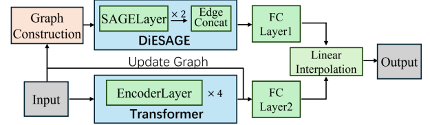
Fig. 4. The module-level overview of BPF-DAG.
