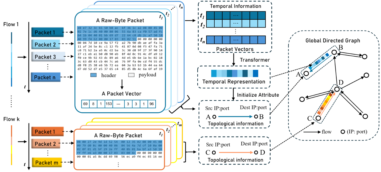
Fig. 2. The schematic illustration of flow preprocessing.
