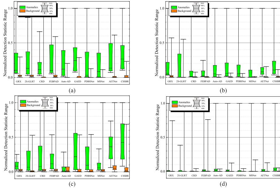
Fig. 7. Separability maps for different methods on four datasets. (a) Pavia. (b) Texas Coast. (c) Cri. (d) EI Segundo.
