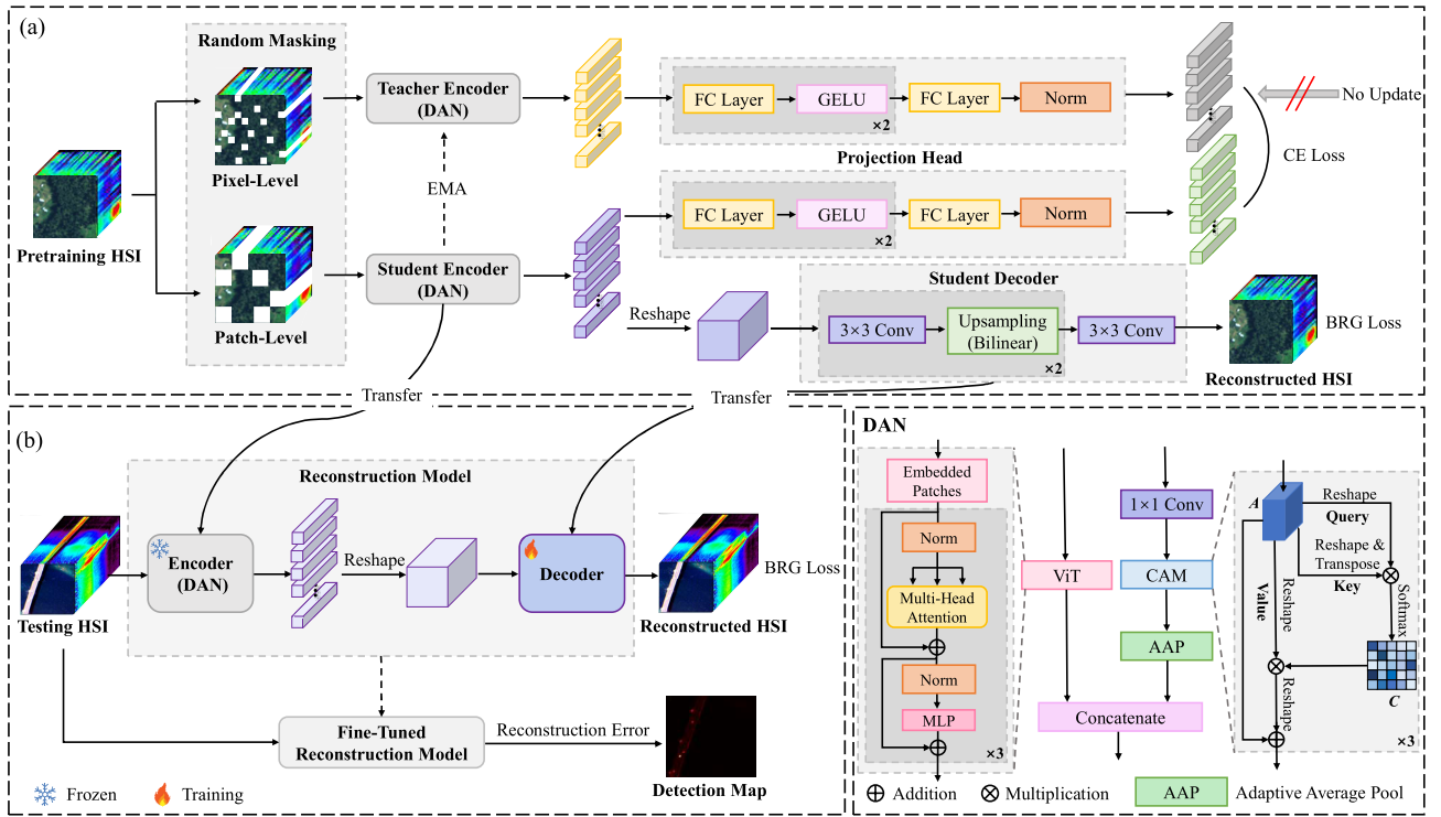
Fig. 1. Overall architecture of the proposed CSSBR method. (a) Pretraining. (b) Transferring to HAD.
