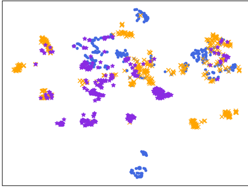
Fig. 13. Visualization of known classes (blue circle), new classes (orange cross), and negative samples filtered from unlabelled data (purple pentagon) on MixD1.
