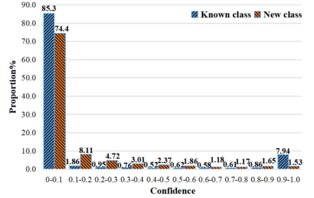
Fig. 5. Confidence distributions of known and new classes.
