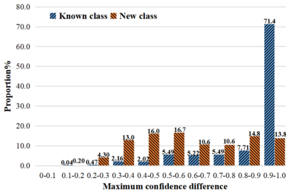
Fig. 6. CfDmax distributions of known and new classes.
