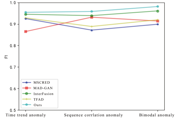
Fig. 7. F1 score of model in three abnormal modes of ASD dataset
