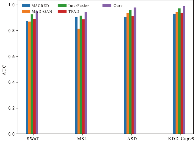
Fig. 6. The AUC values comparison of models
