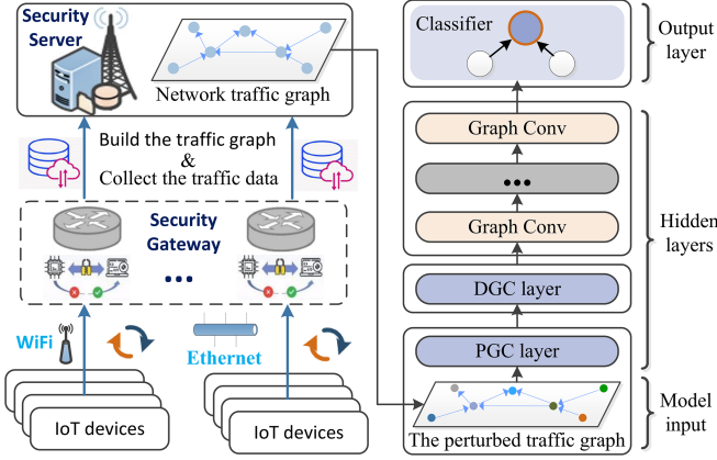
Fig. 4. An overview of NIGNN architecture.
