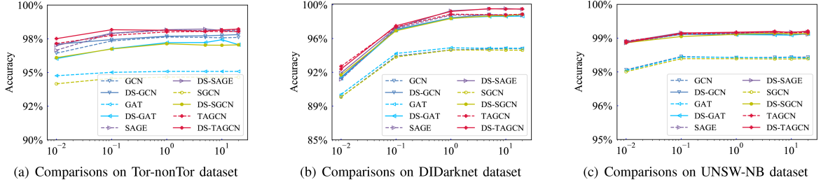
Fig. 10. Experimental results of different graph-based model comparisons under varying privacy budgets \epsilon .
