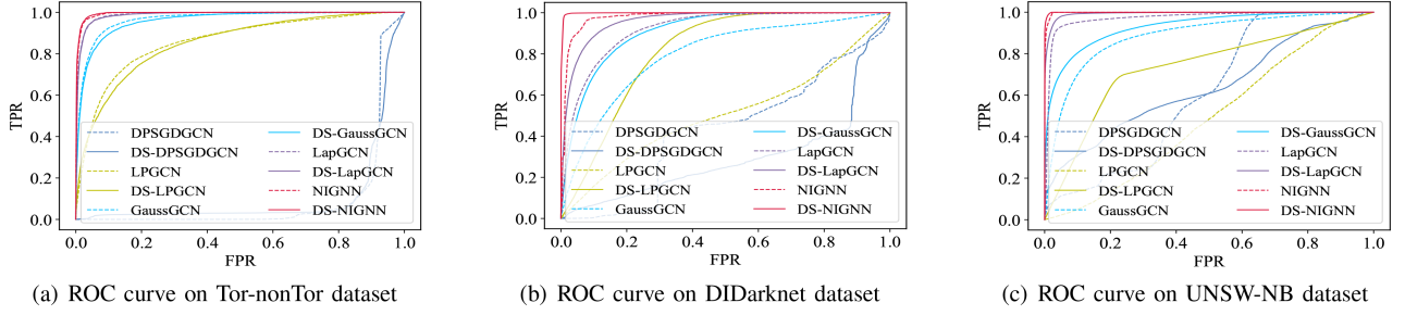
Fig. 7. ROC curve of NIGNN versus private-preserving methods on three benchmark datasets.
