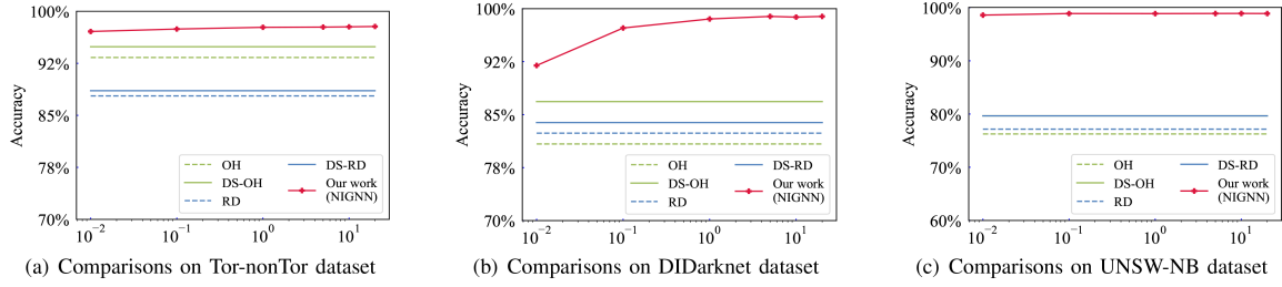
Fig. 8. Experimental results of different feature comparisons under varying privacy budgets \epsilon .
