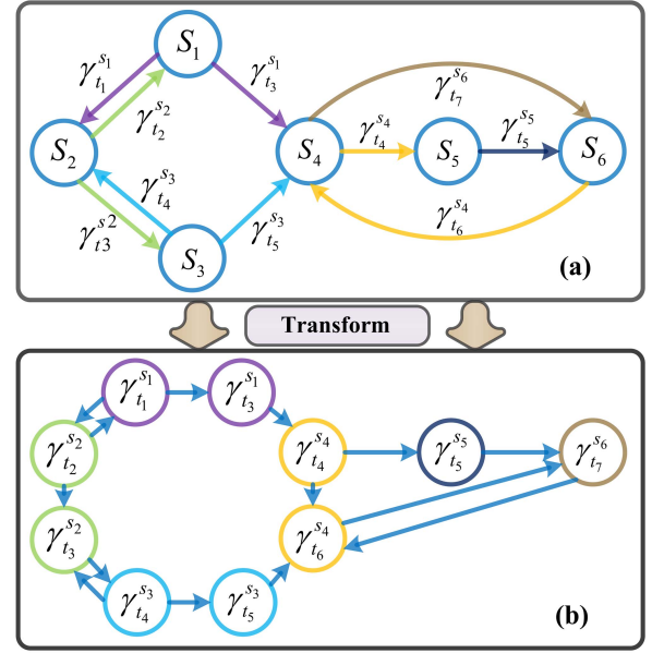
Fig. 3. Details of graph transformation.
