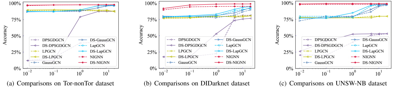
Fig. 6. Experimental results of different private-preserving method comparisons under varying privacy budgets \epsilon .
