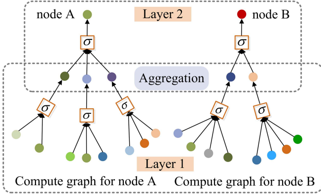
Fig. 1. Details of message passing.
