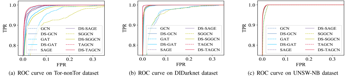
Fig. 11. ROC curve of NIGNN versus graph-based models on three benchmark datasets.
