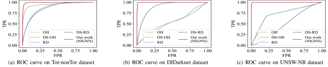
Fig. 9. Experimental results of different feature comparisons.
