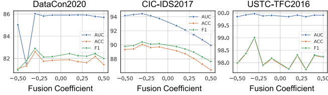
Fig. 9. Experience on the coefficient \beta for anomaly awareness fusion.
