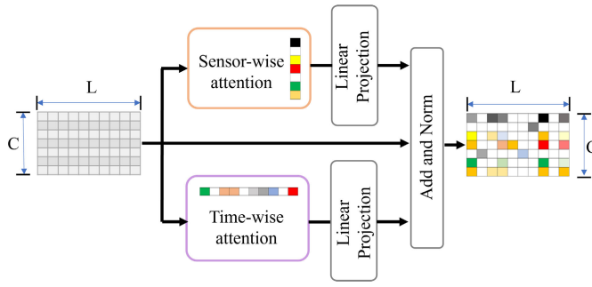
Fig. 4. Dual-channel attention mechanism (DAM).
