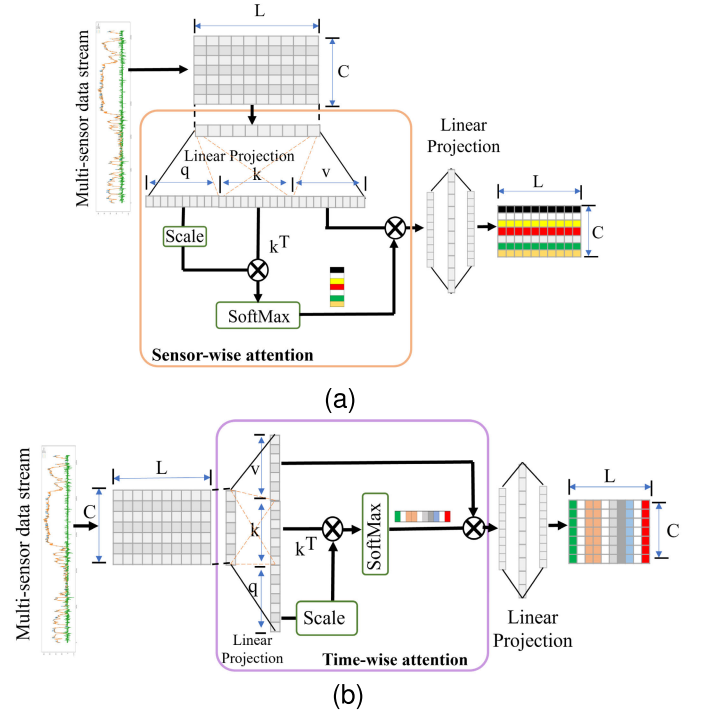
Fig. 5. (a) Sensor-wise attention. (b) Time-wise attention.
