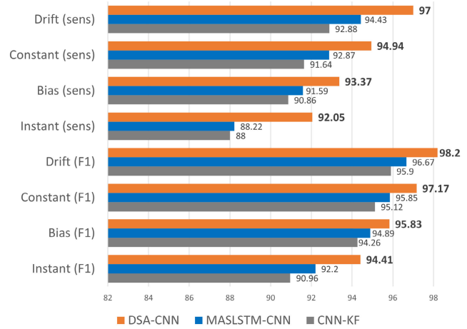
Fig. 6. Performance comparison of different models for single anomaly detection.
