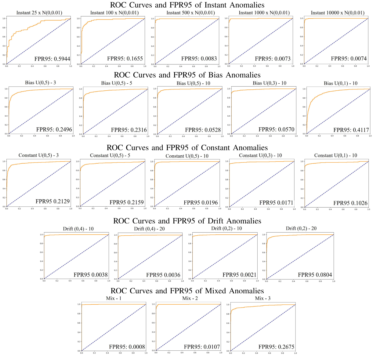
Fig. 7. ROC curves and FPR95 metrics of the experiments conducted in this study.
