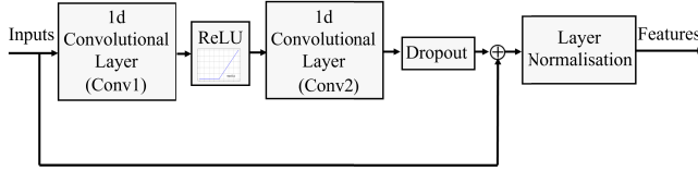
Fig. 3. CNN block.
