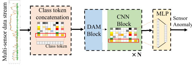
Fig. 2. Architecture of dual-channel self-attention-based convolutional neural network (DSA-CNN) for sensor anomaly detection.
