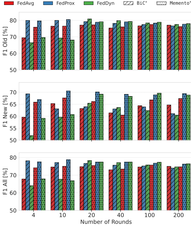
Fig. 4. Comparison of different FL approaches for TON_IoT with expanded feature set in the S_1 scenario.
