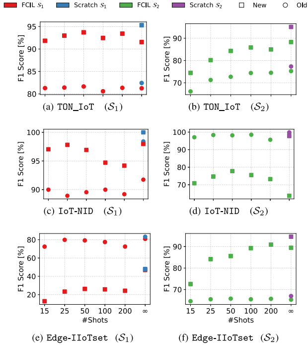
Fig. 8. Performance under few-shot conditions (ranging from 15 to 200 samples) and with all samples ( +\infty ) for the best FCIL method and Scratch , in both few-client and many-client scenarios using the best seed.
