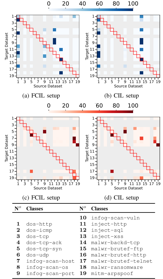
Fig. 7. Confusion matrices for NIDS trained on TON_IoT (source dataset) and evaluated on Edge-IIoTset (top row) and IoT-NID (bottom row) in S_1 . Gray-shaded rows and columns indicate classes that are absent in the target or source dataset.
