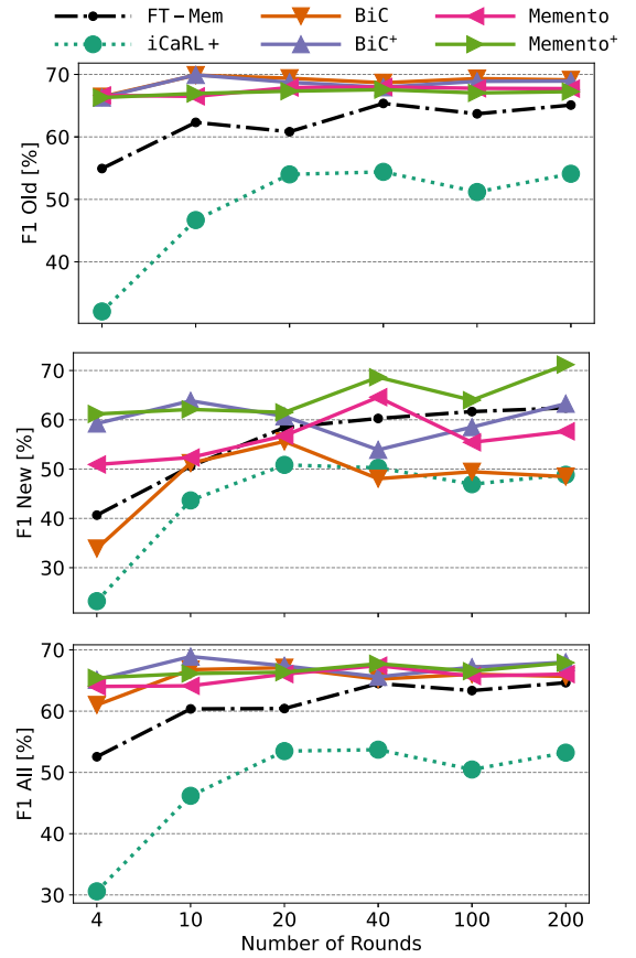
Fig. 3. FCIL performance on TON_IoT in the \mathcal{S}_1 scenario with the base feature set. Different line styles distinguish approaches according to the mitigation strategies employed.
