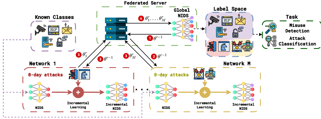
Fig. 1. Visual representation of the overall proposal. Each client incrementally trains its local NIDS, including new attacks, and simultaneously participates in the federated network's collaborative information exchange. This process converges to a global NIDS, then distributed across all clients, to perform (binary and multiclass) misuse detection and attack classification.
