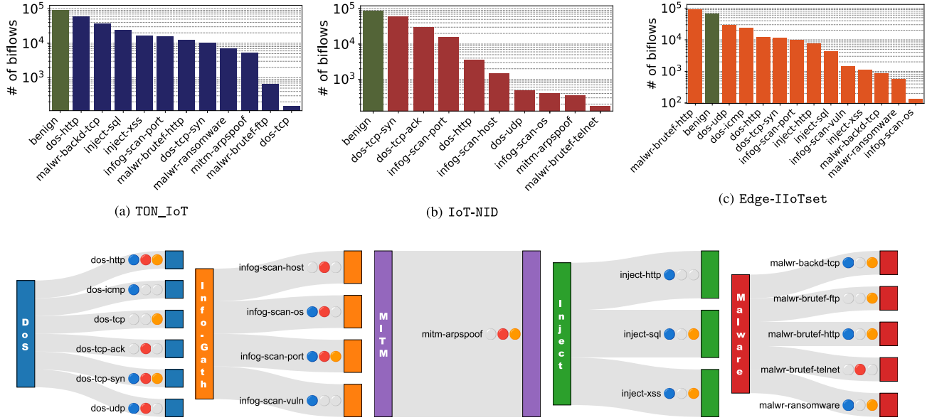
Fig. 2. Biflows distributions for the IoT datasets employed. Green bars represent the benign class across all three datasets. Sankey diagrams show specific attacks per category, with colored circles indicating the datasets that contain each attack.
