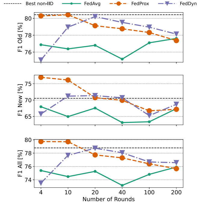
Fig. 6. Comparison of different FL approaches for TON_IoT on new IID data, alongside the best non-IID configuration.
