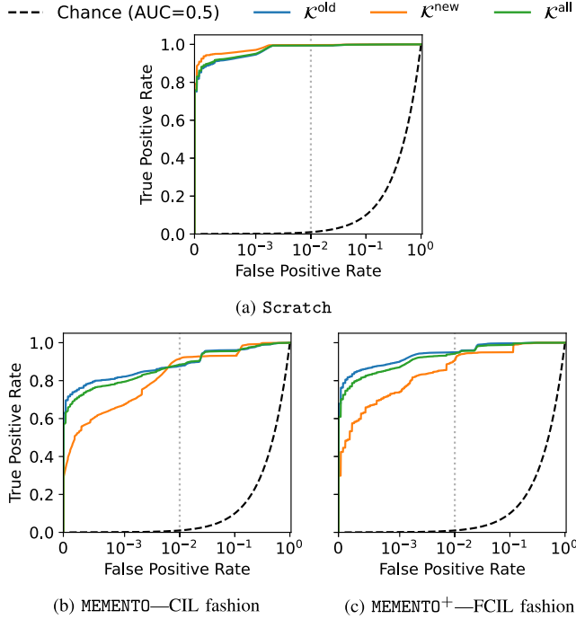
Fig. 5. ROC curves for (a) Scratch, (b) MEMENTO, and (c) MEMENTO + in the S_1 scenario on the TON_IoT dataset. Curves are averaged across all the seeds. The x-axis is displayed in a symlog scale for improved visibility.
