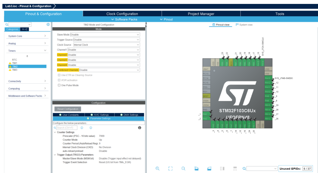
Hình 1.12: STM32 project setting for traffic light application
