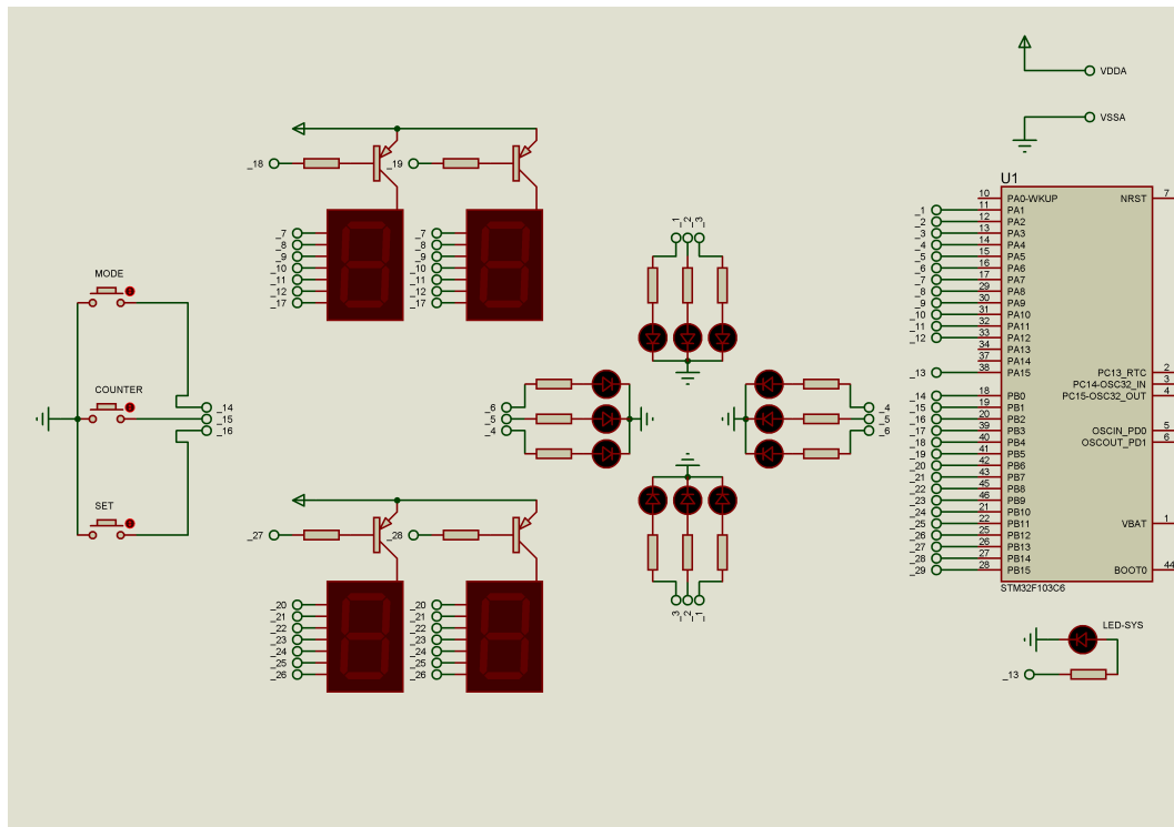
Hình 1.11: Proteus schematic for traffic light application
