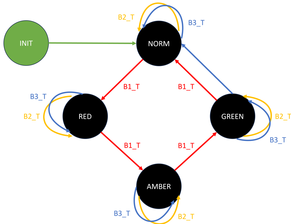
Hình 1.10: An FSM for traffic light application
