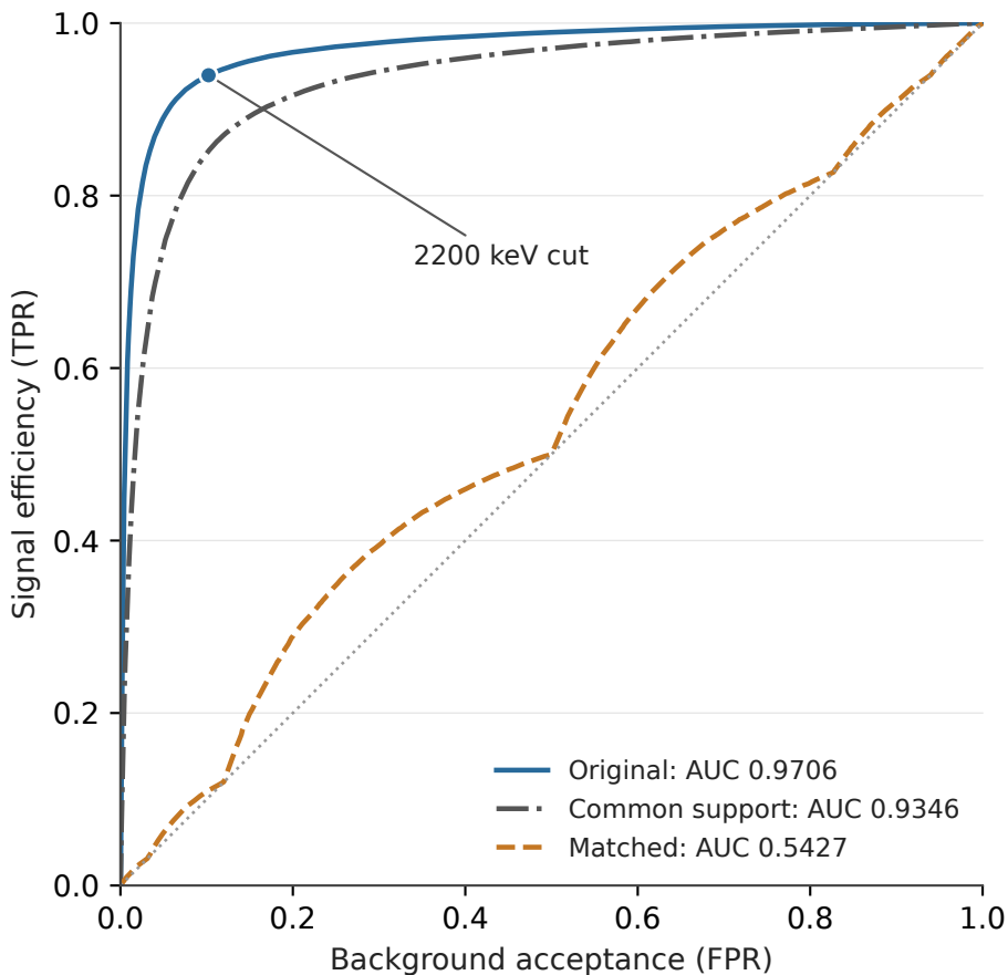
EnergyBench: energy-only ROC SuperNEMO 0\nu\beta\beta vs ^{214}\text{Bi} ; same score s = E_1 + E_2
