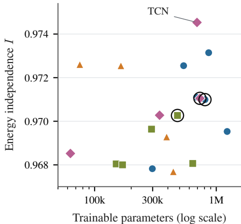
(b) Energy independence \uparrow
