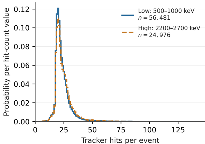
(a) ^{214}\text{Bi}
