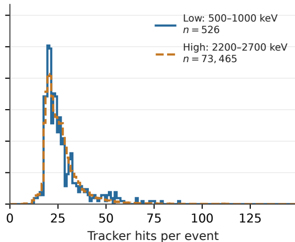
(b) 0\nu\beta\beta
