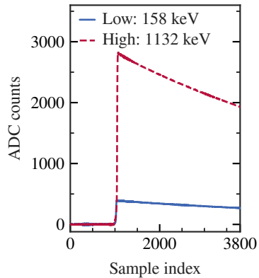
(a) MJD waveforms
