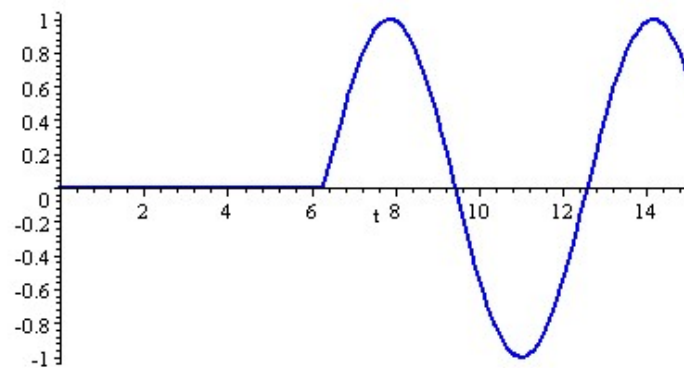
Figure 125: The \sin t portion starts at t = 2\pi because we have multiplied \sin t by u(t - 2\pi)
