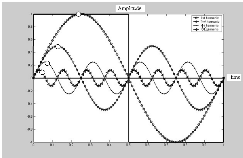
Figure 74: Time domain
