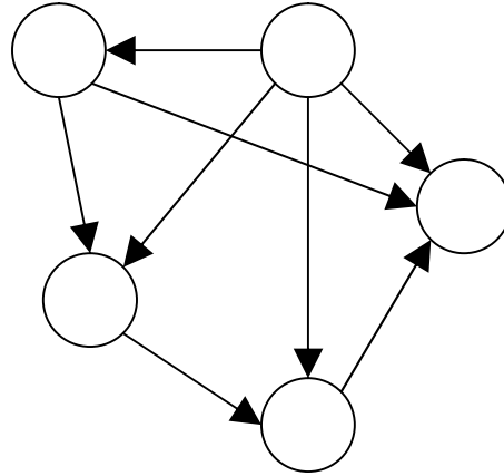
Figure no 40: Not Strongly Connected
