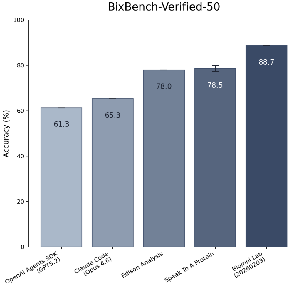
Figure 3: Accuracy on BixBench-Verified-50. Baseline scores are reproduced from the public leaderboard; error bars for Speak to a Protein indicate variability across repeated runs.
