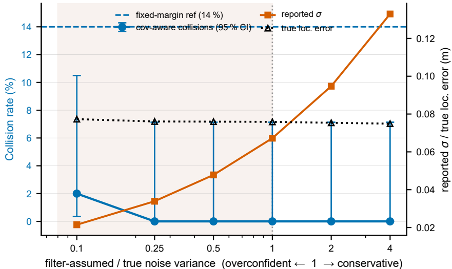
Robustness to filter (in)consistency
