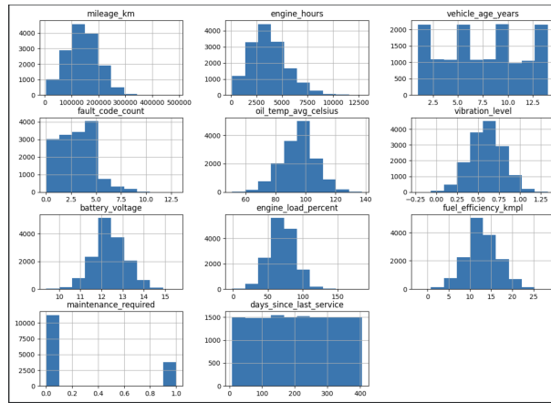
Figure 1: Values Range
