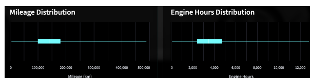
Figure 3: Box Plot
