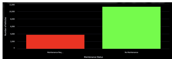
Figure 2: Class Imbalance
