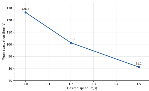
FIGURE 12. Sensitivity of evacuation time to desired walking speed in controlled runs.
