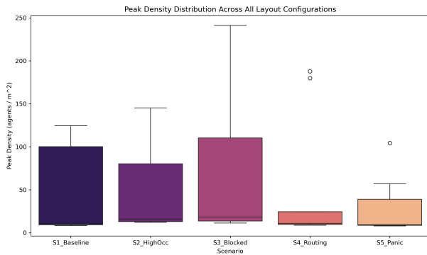
FIGURE 18. Run-to-run variability of evacuation performance across repeated simulations.
