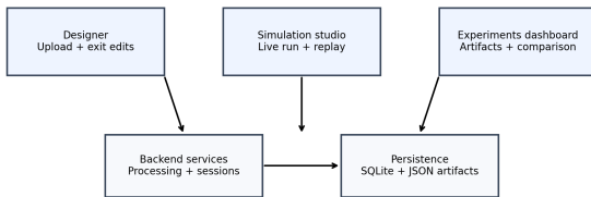
FIGURE 5. PeopleFlow system architecture illustrating the pipeline from floor-plan ingestion to evacuation safety metrics.
