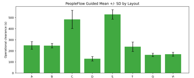
Fig. 10. Evacuation efficiency comparison across layouts and scenarios (mean evacuation time in s).
