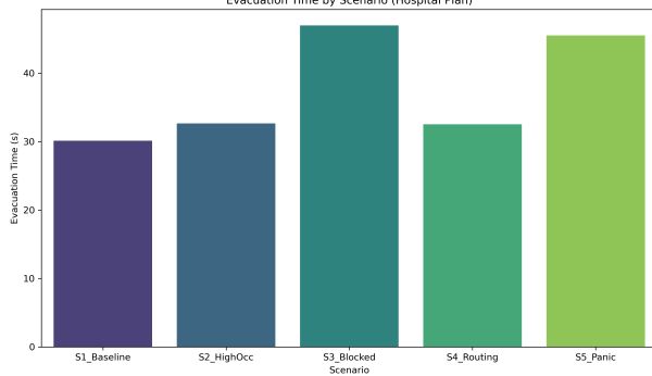
Evacuation Time by Scenario (Hospital Plan)
