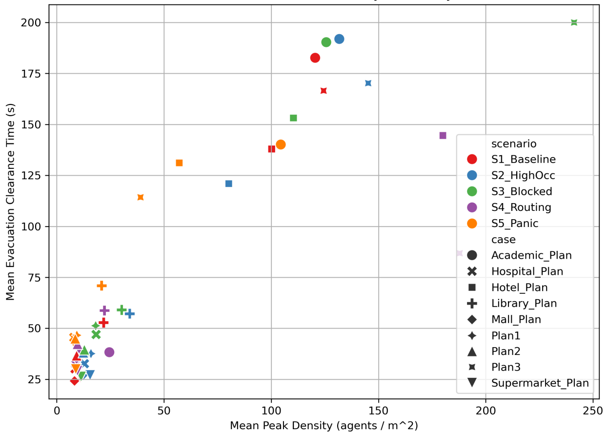
Evacuation Time vs Peak Density across Layouts
