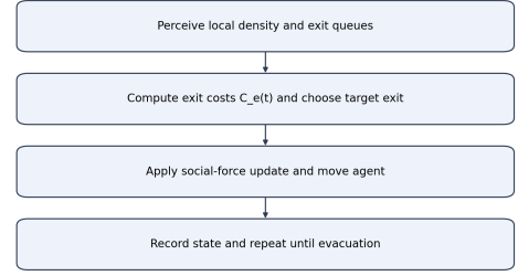
FIGURE 1. Agent movement logic used in each simulation step.
