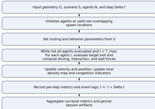
FIGURE 4. PeopleFlow simulation loop.
