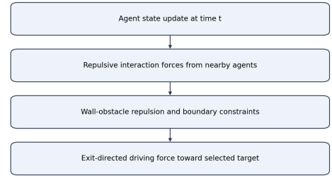
FIGURE 2. Social-force interaction components used for each movement update.
