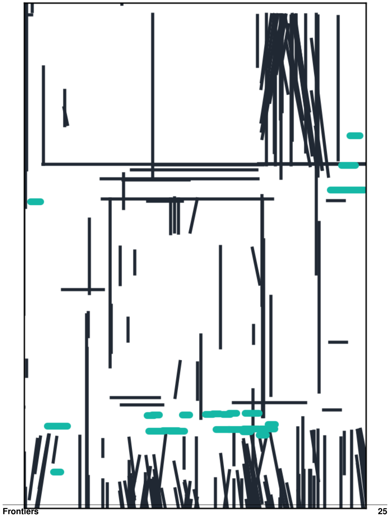
Figure 8. Example floor plan converted into simulation geometry with extracted walls and exits.
