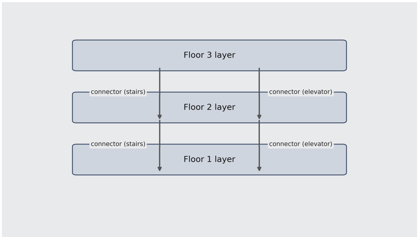
Figure 20. Conceptual layered 3D routing extension with inter-floor connectors.
