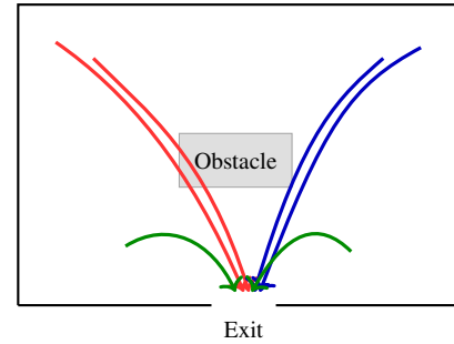
Fig. 12. Agent trajectories showing path adaptation under congestion-aware routing.
