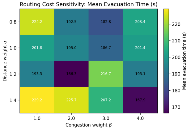
Fig. 8. Sensitivity heatmap of routing weights \alpha and \beta (mean evacuation time in s).
