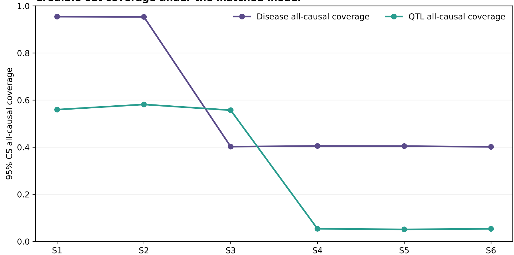
Credible-set coverage under the matched model
