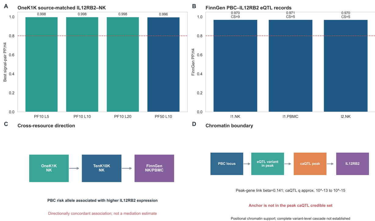
Figure 4. IL12RB2–NK is supported across molecular-QTL resources within bounded causal claims. (A) OneK1K best signal-pair PP.H4 across PF10/PF50 and L configurations. (B) FinnGen PBC–IL12RB2 molecular-QTL records. (C) Direction of the PBC risk allele across OneK1K, TenK10K and FinnGen. (D) Positional chromatin evidence and the missing variant-level caQTL credible-set link. The diagram does not assert a complete causal cascade. Abbreviations: caQTL, chromatin-accessibility quantitative-trait locus; eQTL, expression quantitative-trait locus; L, maximum SuSiE effects; PF, expression-factor model.
