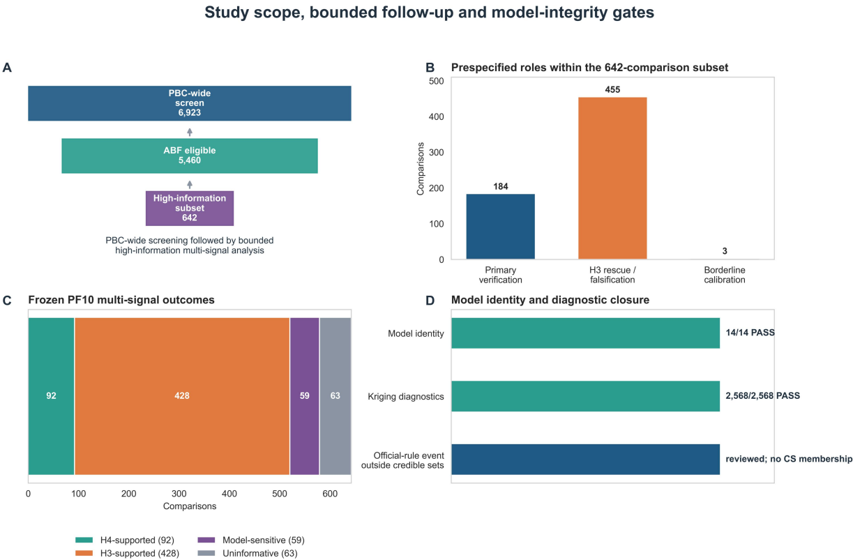
Figure 1. Study scope, bounded follow-up and model-integrity gates. (A) Flow from the 6,923-comparison PBC-wide registry to 5,460 ABF-eligible comparisons and the frozen 642-comparison multi-signal subset. (B) Prespecified roles within the subset. (C) Final PF10 multi-signal comparison states. (D) Current-release source identity and corrected kriging diagnostic closure. The official-rule event was reviewed and did not enter a credible set. Abbreviations: ABF, approximate Bayes factor; CS, credible set; H3, distinct-signal-pair support; H4, shared-signal-pair support; PF10, model using ten expression factors.
