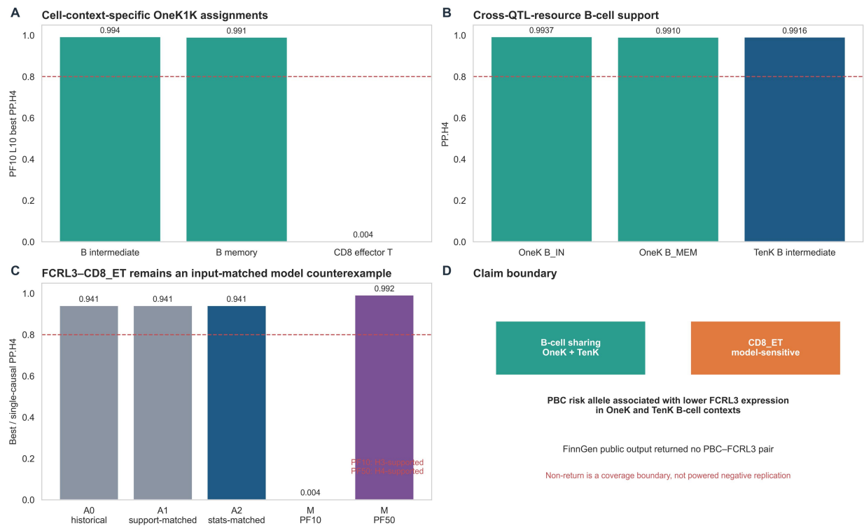
Figure 5. FCRL3 combines reproducible B-cell sharing with a T-cell model-sensitivity counterexample. (A) OneK1K PF10 best signal-pair PP.H4 for representative cells. (B) Cross-QTL-resource B-cell support. (C) FCRL3-CD8_ET across matched-input ABF arms and PF10/PF50 multi-signal configurations. (D) Claim boundary for direction and FinnGen coverage. Abbreviations: B_IN, intermediate B cell; B_MEM, memory B cell; CD8_ET, effector CD8 T cell.
