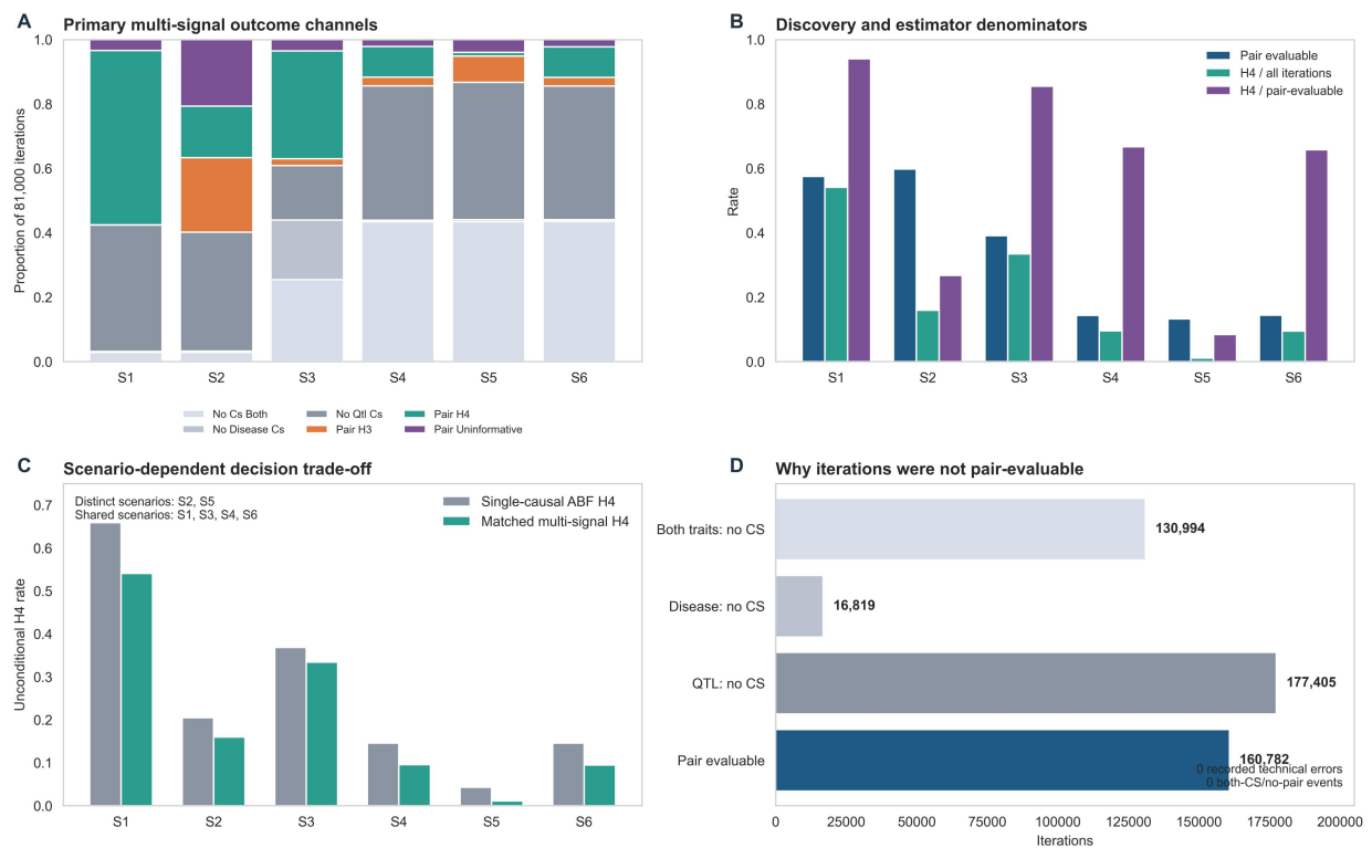
Figure 3. Simulation separates credible-set discovery from pair-conditional inference. (A) Primary multi-signal outcome channels by scenario. (B) Pair-evaluable, unconditional H4 and pair-conditional H4 rates. (C) Unconditional ABF and matched multi-signal H4 rates; S2 and S5 are distinct-signal scenarios. (D) Aggregate discovery channels. The primary branch had no recorded technical errors and no both-CS/no-pair events.
