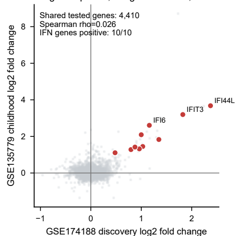
c Program-specific, not genome-wide, coherence
