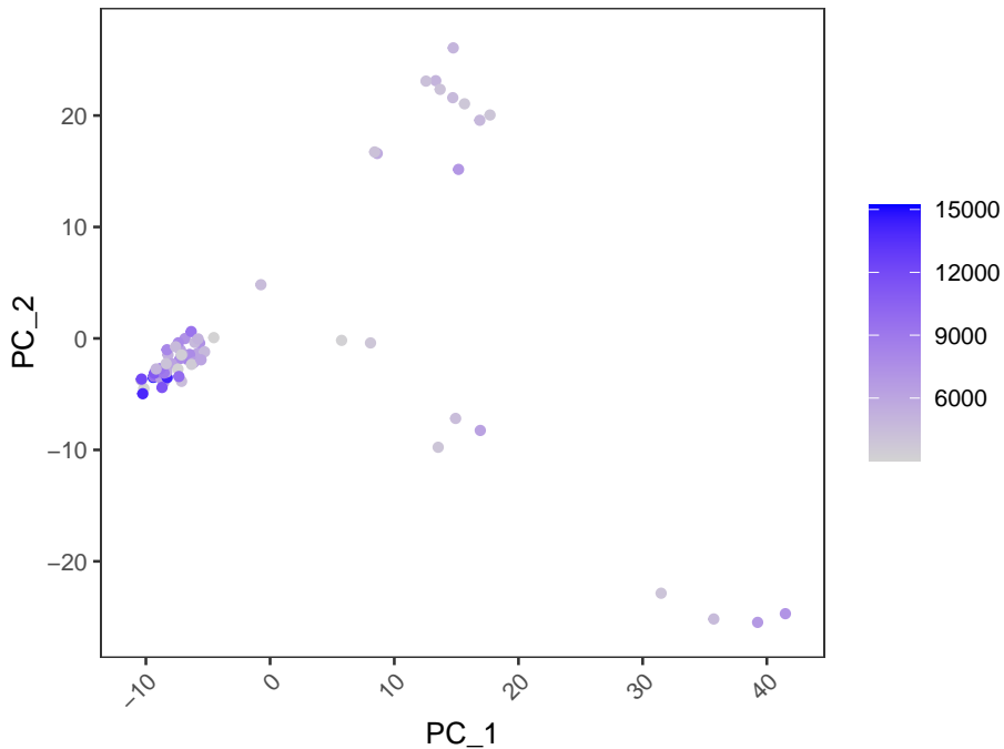
House Beta ... PCA (PC1 vs PC2, coloured by nCount_RNA)
