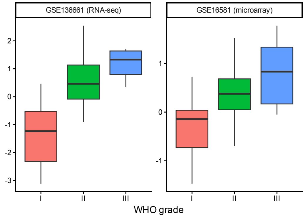
Program score increases with grade (cross-cohort)
