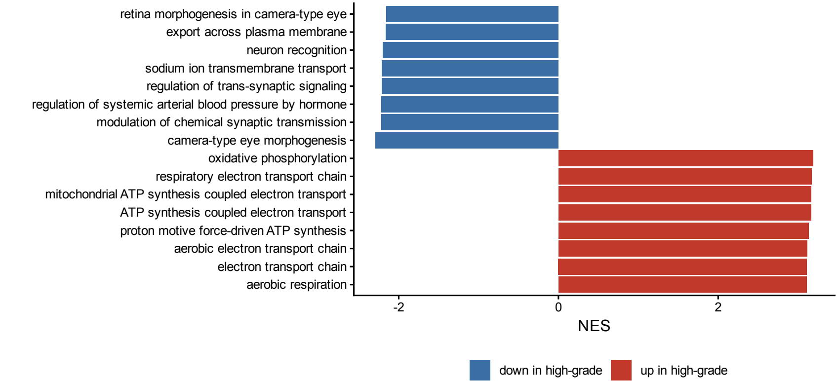
GSEA: OXPHOS/ribosome up, synaptic/Wnt down
