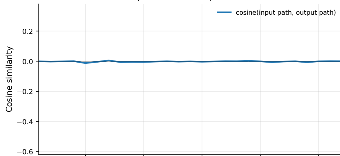
S12 input shift + multiplicative LoRA
