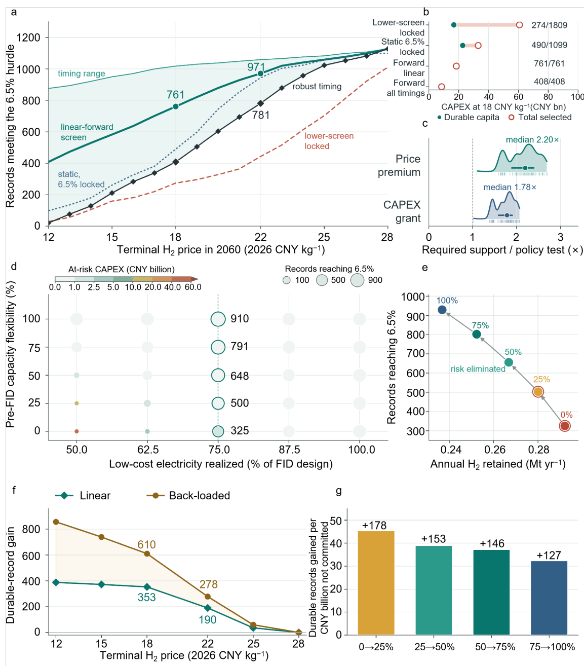
Fig. 4 Price-informed screening and pre-investment capacity flexibility move exposure ahead of capital lock-in. a , Records remaining above 6.5% under alternative commitment rules across conditional terminal prices of 12–28 CNY kg -1 ; the green band spans front-loaded to back-loaded timing, the heavy line denotes the linear path and black diamonds denote timing-robust screening. b , Durable and total selected capital under four commitment rules for the linear 18 CNY kg -1 path; right-hand labels give durable/selected records. c , Required 15-year price premiums and upfront capital grants normalised by illustrative policy tests; ridges show distributions, thick lines show interquartile ranges and circles mark medians. d , At-risk capital under the primary 1-MW minimum-build convention across resource realisation and pre-FID adjustability; colour gives at-risk capital, circle area gives records reaching 6.5%, and outlines and adjacent values identify the 75% resource slice. e , Continuous-downsizing trade-off at 75% resource realisation between annual hydrogen retained and records reaching 6.5%; labels give adjustability and coral outlines identify cases with residual exposure. f , Additional durable records retained by linear and back-loaded rather than timing-robust screening across terminal prices; front-loaded timing yields no gain. g , Marginal durability yield of each 25-percentage-point increase in continuous pre-FID adjustability at 75% resource realisation. Each step releases the same 3.93 billion CNY of planned CAPEX from commitment. Bars report the additional records reaching 6.5% per CNY billion not committed, and labels above bars give the corresponding record gains; declining bar heights therefore indicate diminishing marginal durability gains per equal capital increment.
