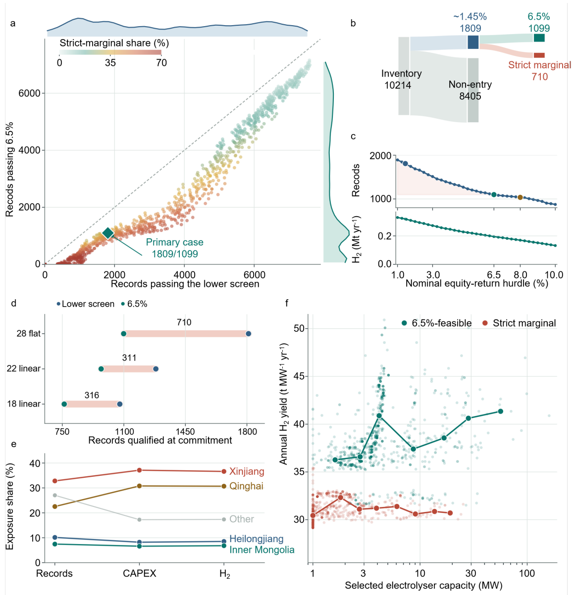
Fig. 2 Return criteria create a continuous and information-dependent qualification boundary. a , Records passing the lower and 6.5% screens across 972 deterministic constrained-electricity configurations; colour gives the strict-marginal share, marginal curves show the distributions and the diamond marks the primary case. The configurations are an unweighted sensitivity ensemble, not a probability distribution. b , Flow from the 10,214-record inventory to static lower-rule qualification, non-qualification, 6.5%-qualified and strict-marginal cohorts. c , Qualified records and annual hydrogen after independent resizing across a continuous 1–10% nominal equity-return frontier; highlighted points mark the lower rule, 6.5% and 8%. d , Paired qualification under a static 28 CNY kg -1 reference and linear 22 and 18 CNY kg -1 paths anticipated at commitment; coral spans give the strict-marginal cohort. e , Provincial shares of strict-marginal records, gross installed-system capital and annual hydrogen output. f , Record-level electrolyser capacity and annual hydrogen yield for 6.5%-feasible and strict-marginal records; heavy lines and large points trace bin medians.
