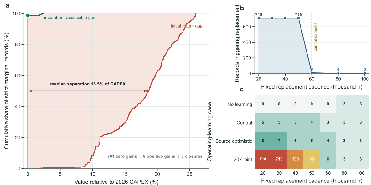
Fig. S4 Replacement timing separates physical access to operating learning from the sufficiency of its financial payoff. a , Empirical cumulative distributions of the initial 6.5% NPV gap and central replacement-mediated operating gain across 710 strict-marginal records on the same 2026-CAPEX scale. b , Records triggering at least one replacement over 30 years under fixed replacement cadences; the dashed line marks the central 60,000-hour assumption. c , Records reaching 6.5% under no learning, central learning, source-informed optimistic learning and a twenty-fold joint-improvement stress. At 80,000–100,000 hours no record replaces; the three classifications above 6.5% therefore reflect avoided replacement expenditure rather than captured learning. All cases are deterministic counterfactuals.
