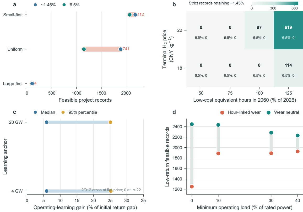
Fig. S2 High-risk boundary tests separate uncertainty in exact cohort size from robustness of the return-separation mechanism. a , Low-return and 6.5%-feasible records under province–technology energy-conserving allocation extremes; coral spans are strict-marginal cohorts and labels give their sizes. b , Strict-marginal records retaining the low-return criterion under linear lifetime resource-access paths and terminal producer prices; every cell has zero durable 6.5% upgrades. c , Median and 95th-percentile incumbent-learning gains relative to initial return gaps when cumulative global electrolysis is anchored at 4 or 20 GW; the arrow locates the out-of-range 100% closure boundary. d , Low-return entry across alkaline minimum-load assumptions with standard hour-linked degradation and replacement accounting or a wear-neutral counterfactual. All panels use deterministic stress tests and do not represent probability intervals.
