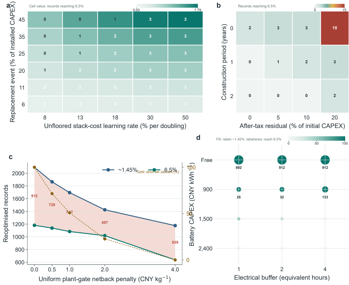
Fig. S3 Boundary tests distinguish robustness of the vintage-learning mechanism from sensitivity of the selected cohort. a , Strict-marginal records reaching 6.5% across unfloored stack-cost learning rates and event replacement-cost shares at a fixed 60,000-h cadence. b , Records reaching 6.5% after adding construction duration and after-tax residual value to the central operating-learning case. c , Reoptimised low-return, 6.5%-feasible and strict-marginal counts under uniform producer-side netback penalties; the line gives Jaccard agreement of strict membership with the zero-penalty cohort. d , Records retaining the low-return criterion and reaching 6.5% under free lossless and costed electrical-buffer cases; the central costed specification uses 1,500 CNY kWh -1 , 85% round-trip efficiency, 15-year life and full replacement. All tests are deterministic boundaries rather than probability estimates.
