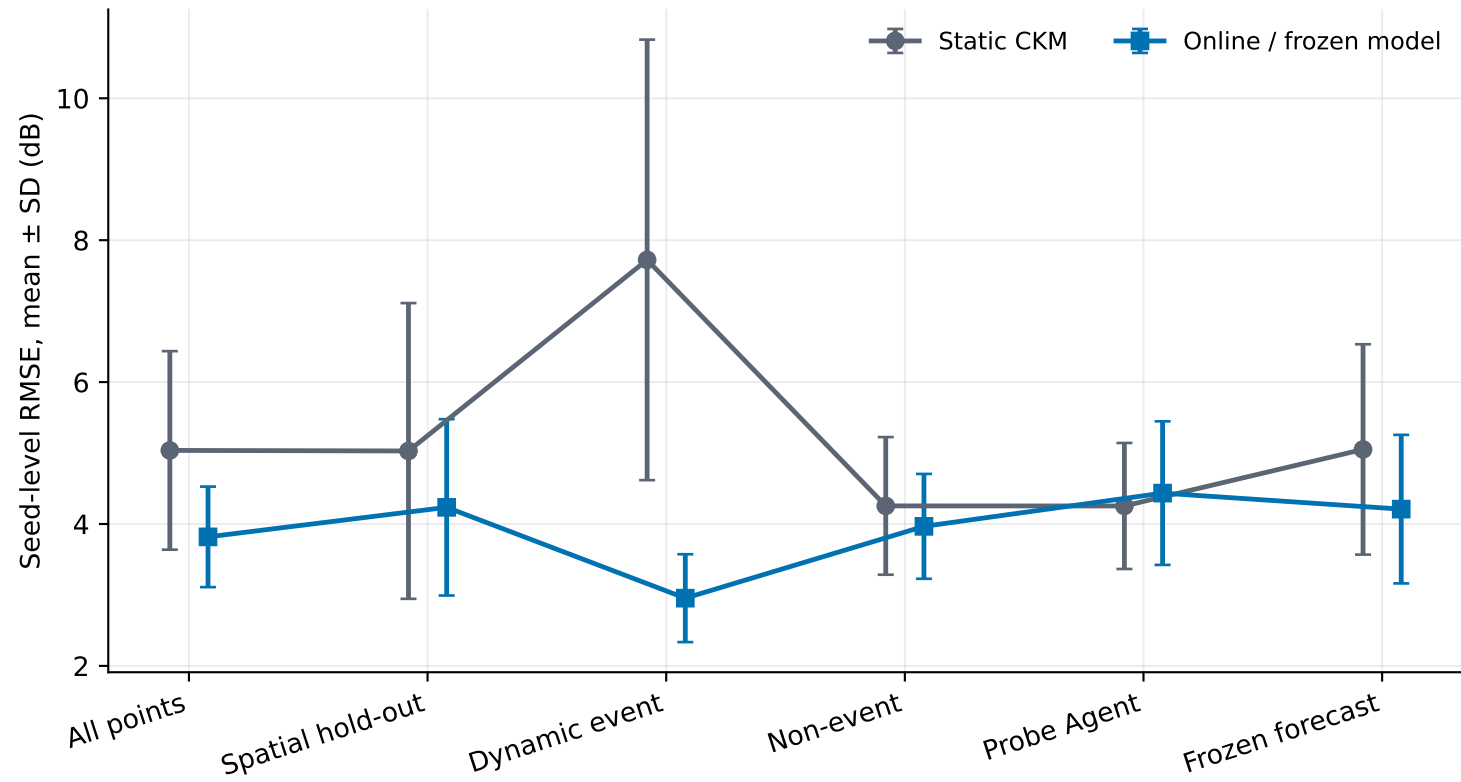
RMSE comparison across evaluation scopes (5 seeds)
