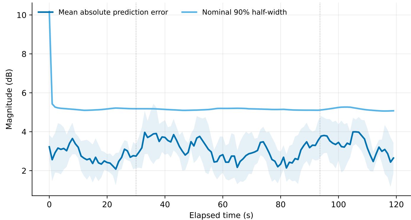
Prediction error and uncertainty over time (5 seeds)
