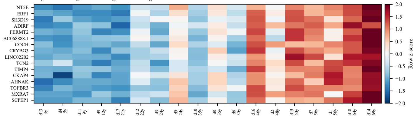
C Representative age-associated genes across age-ordered donors
