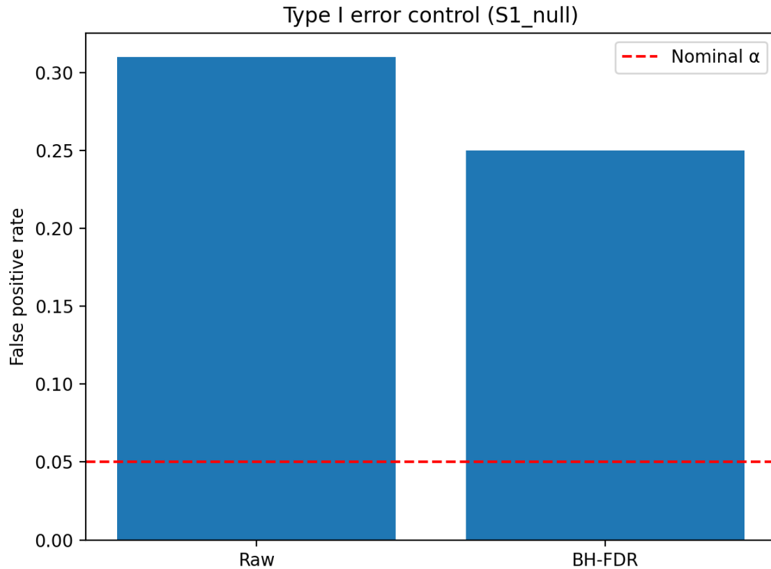
Figure S6 | Type I error control under the null scenario (S1_null).
