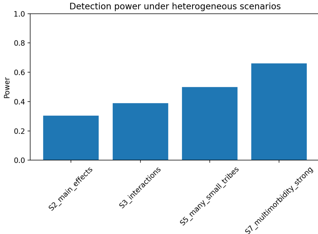
Figure S7 | Detection power under heterogeneous and interaction-driven scenarios.
