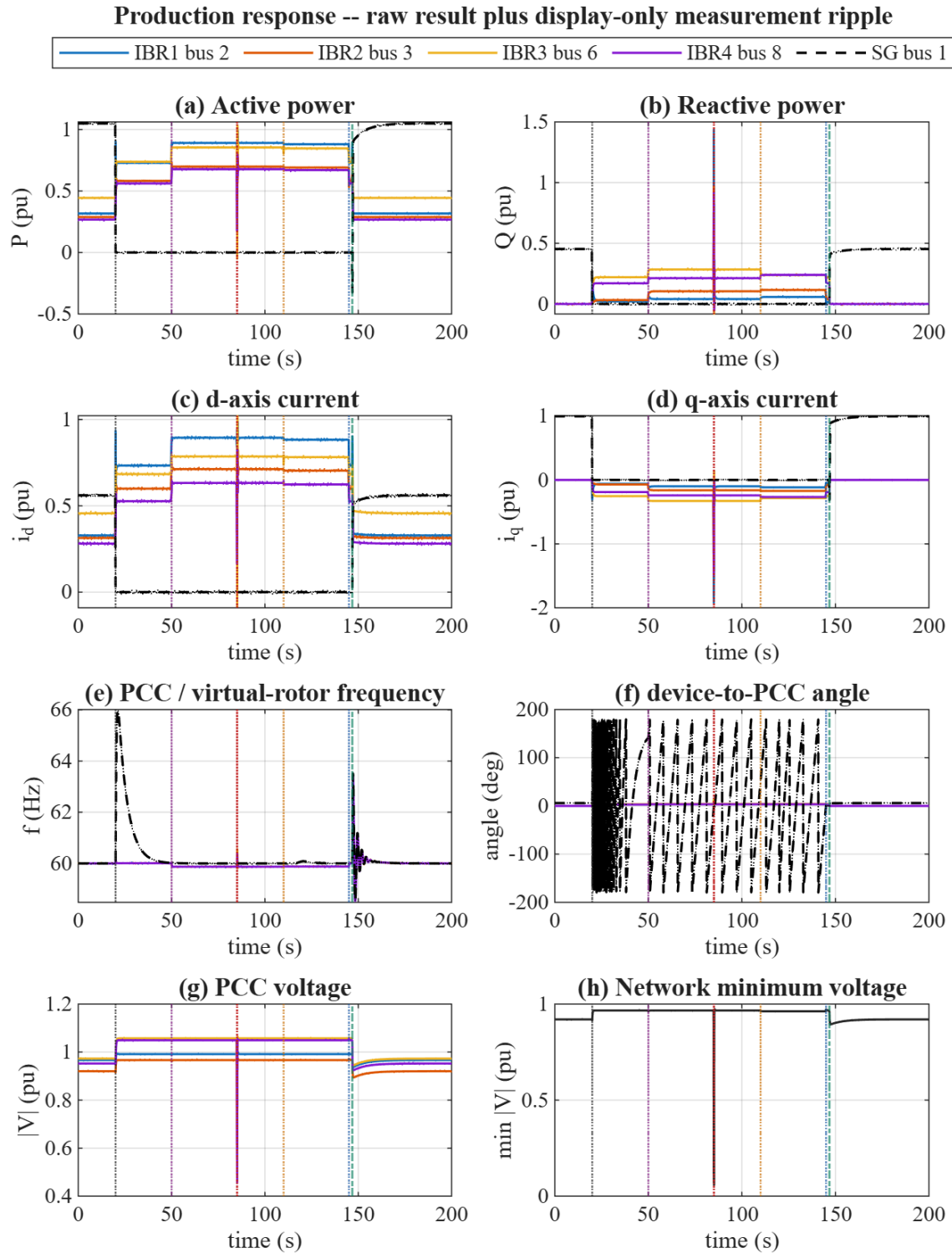
Figure 5: IBR and SG active/reactive power, frame currents, frequency, device-to-PCC angle, PCC voltage, and network minimum voltage. Solid traces are raw production results; dotted band-limited ripple is display-only and does not enter any equation or decision. Remaining vertical event excursions belong to the raw switching transient, not to the ripple.
