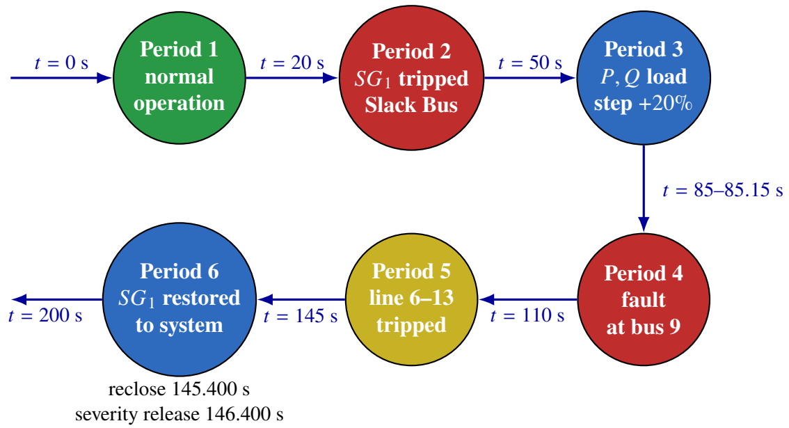
Figure 2: Six-period disturbance sequence of the 200-s simulation from the accepted production event log: normal operation at 0 s, SG trip at 20 s, P, Q load step +20% at 50 s, bus-9 fault 85–85.15 s, line 6–13 trip at 110 s, and topology restoration plus the earliest SG-close request at 145 s. The accepted reclose and later indexed IBR release are separate logged events.
