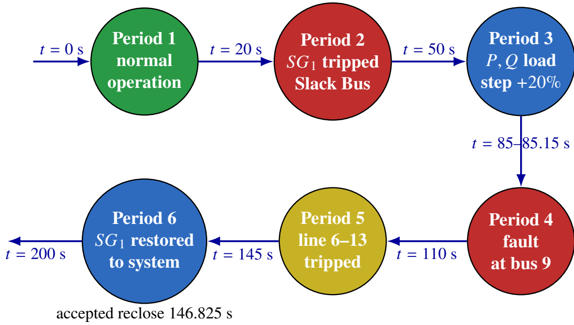
Figure 2: Six-period disturbance sequence of the 200-s simulation from the accepted production event log: normal operation at 0 s, SG trip at 20 s, P, Q load step +20% at 50 s, bus-9 fault 85–85.15 s, line 6–13 trip at 110 s, and SG restoration at 145 s (accepted reclose 146.825 s).
